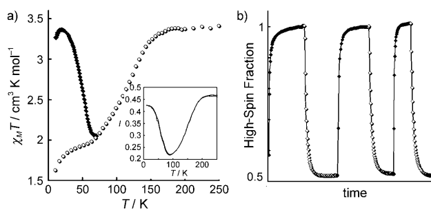
Figure 2. a) Plot of \chi_{\text{M}}T versus temperature per \text{Fe}^{\text{II}} ion (○) and the light-induced excited metastable HS state with subsequent thermal relaxation (◆). The inset shows a plot of optical reflectivity signal versus temperature ( \lambda = 830\text{ nm} ) in the presence of white light. b) Cycling of the green- (◆) and red- (◇) light-induced switching between "on" (HS) and "off" (LS).
